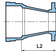
Socket / Flange
