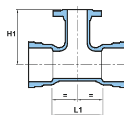
Socket / Flange
