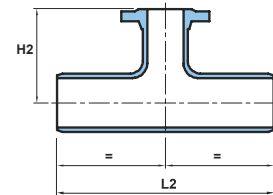
Spigot / Flange
