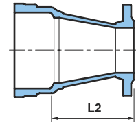
Socket / Flange
