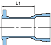
Flange / Socket
