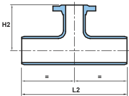
Spigot / Flange
